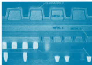
(Reprinted with permission of Integrated Circuit Engineering.) • Actual cross-section of a modern microprocessor chip. Note the multiple levels of metal and planarization.
